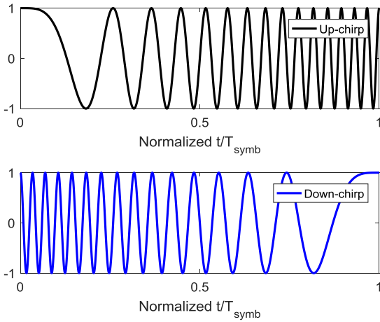
Fig. 2. Up and down chirp signals normalized to T_{symbol} .
